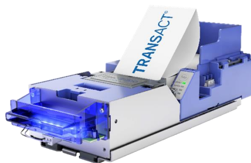
TransAct - Epic Edge™ TITO printer
